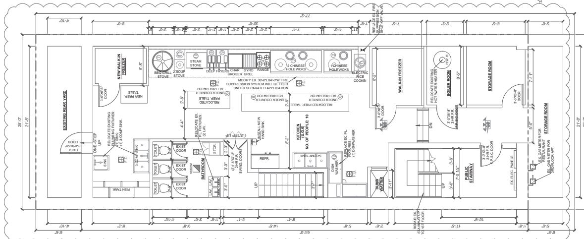
PROPOSED CELLAR PLAN SCALE: 1/4" = 1'-0"
